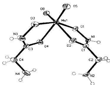
Fig. 6 Crystal structure of [\text{MoO}_2(\text{Glyha})_2] .
