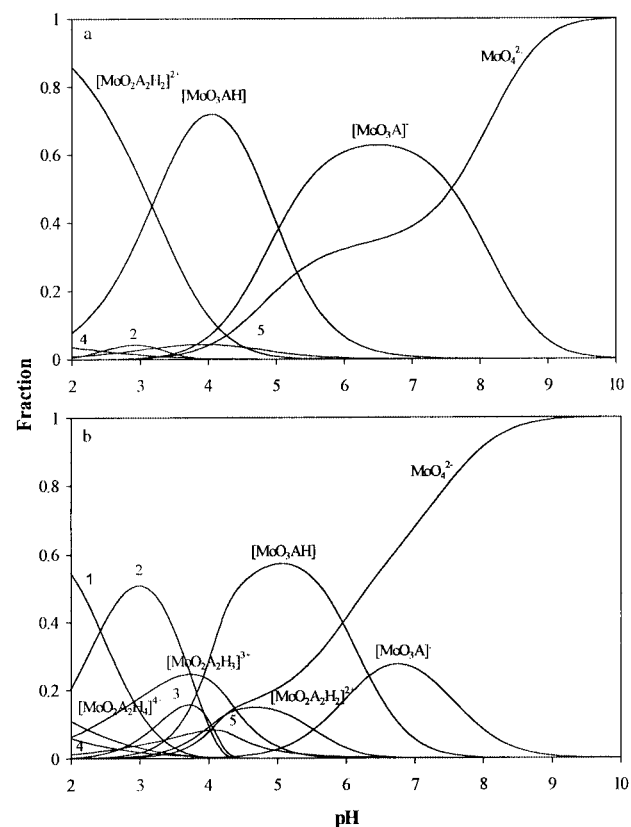
Fig. 3 Concentration distribution curves of complexes formed: (a) in the molybdenum-Sarha system, c_{\text{Sarha}} = 6 \times 10^{-3} \text{ mol dm}^{-3} ; metal to ligand ratio 1:3; and (b) in the molybdenum-Hisha system, c_{\text{Hisha}} = 6 \times 10^{-3} \text{ mol dm}^{-3} ; metal to ligand ratio 1:3. Species 1–5 as in Fig. 2.
